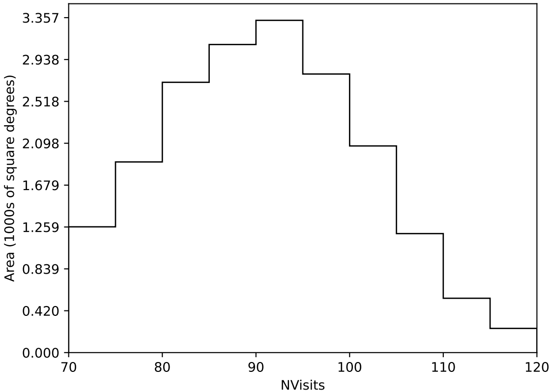
smc_lmc_v3.3_10yrs Yr 1 all bands: NVisits
