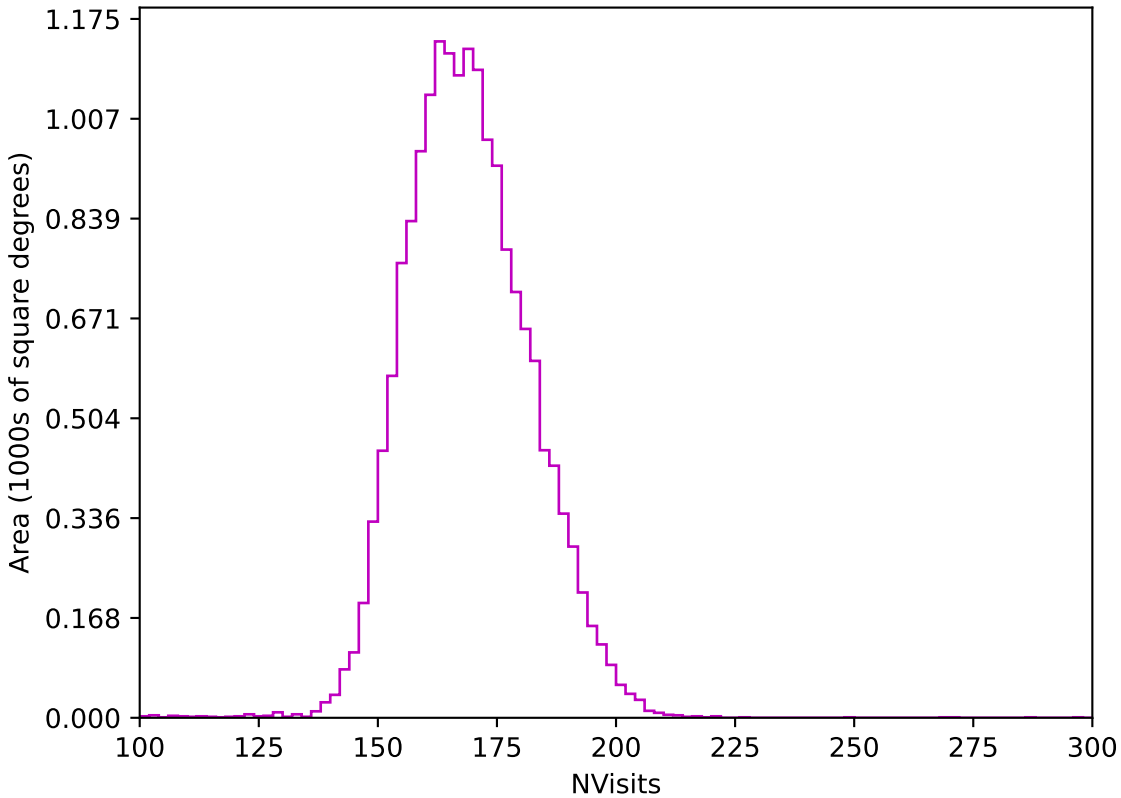
smc_lmc_v3.3_10yrs WFD z band: NVisits
