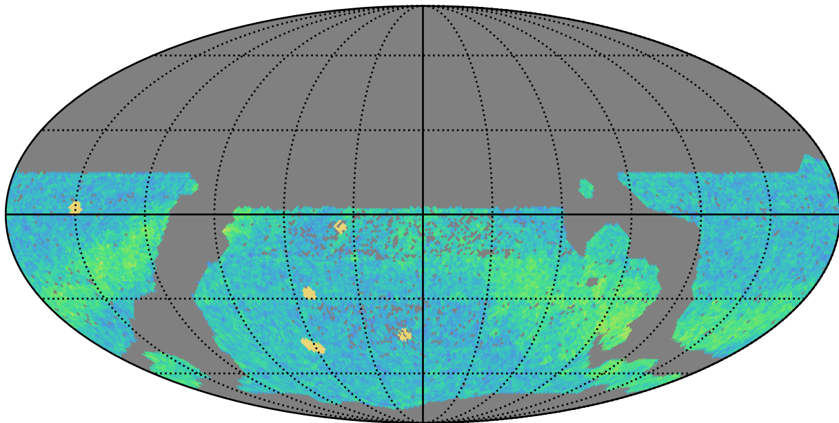
smc_lmc_v3.3_10yrs WFD r band: NVisits
