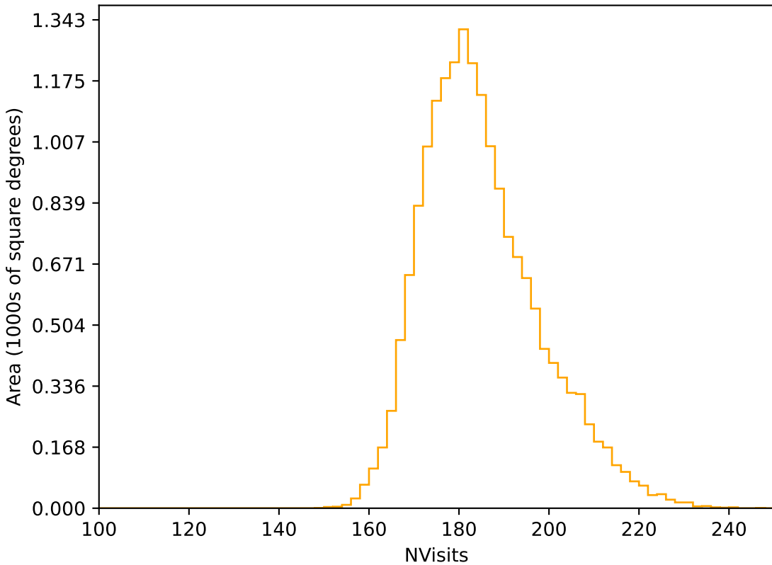
smc_lmc_v3.3_10yrs WFD r band: NVisits
