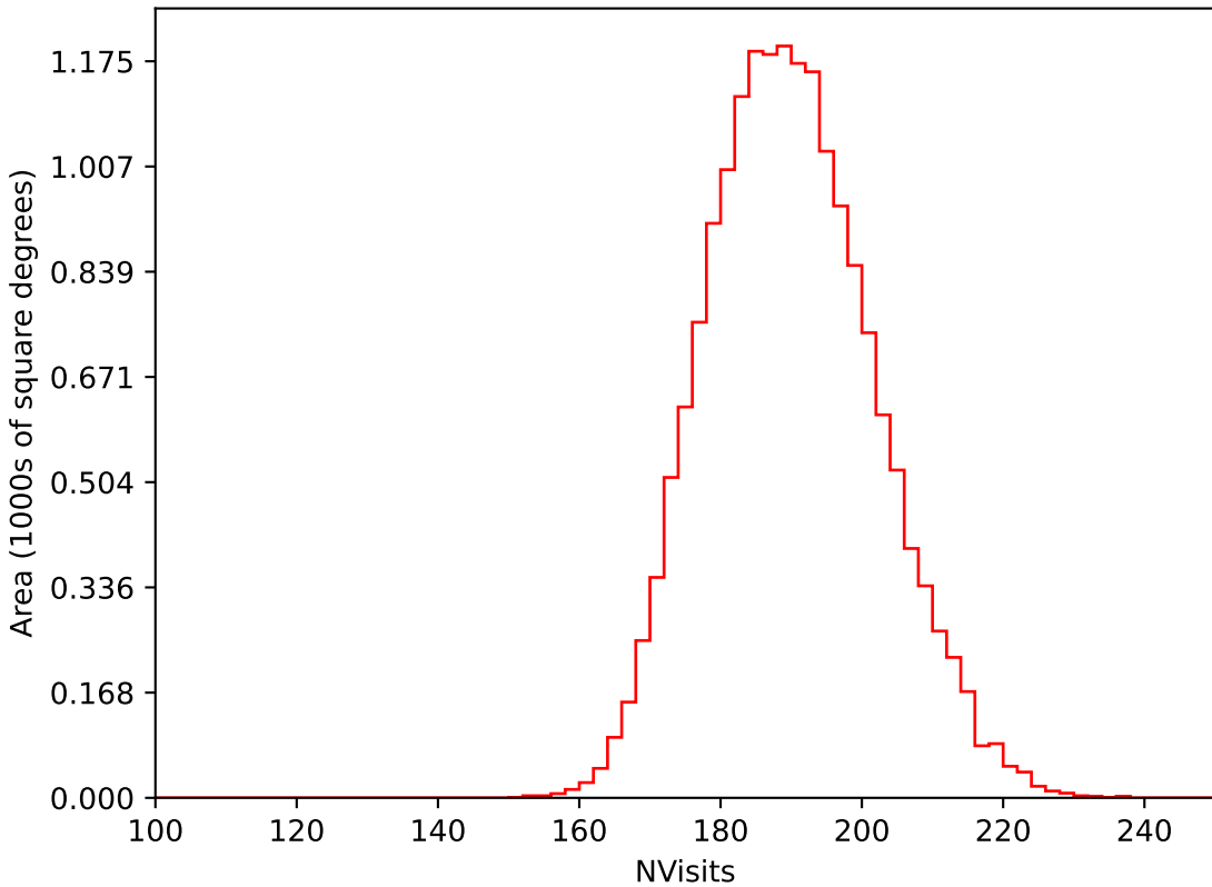
smc_lmc_v3.3_10yrs WFD i band: NVisits
