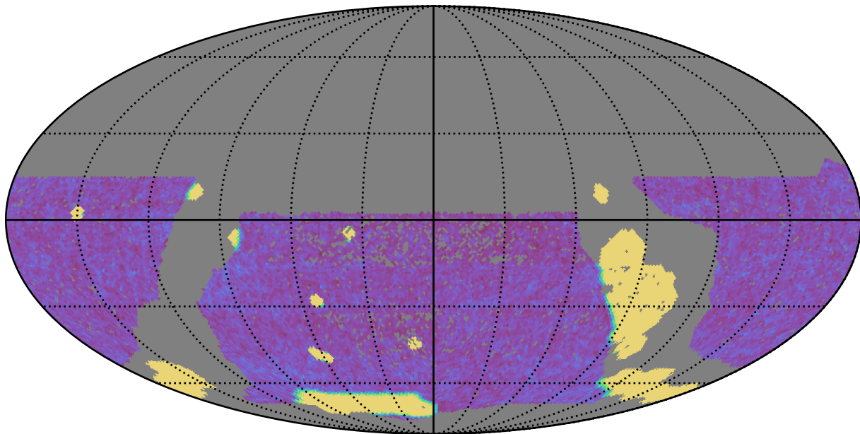
smc_lmc_v3.3_10yrs WFD g band: NVisits
