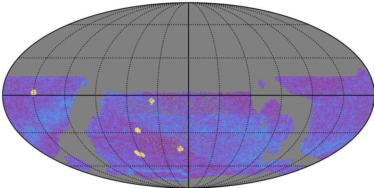
smc_lmc_v3.3_10yrs WFD all bands: NVisits
