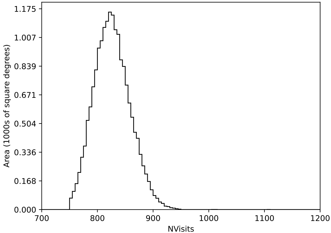
smc_lmc_v3.3_10yrs WFD all bands: NVisits
