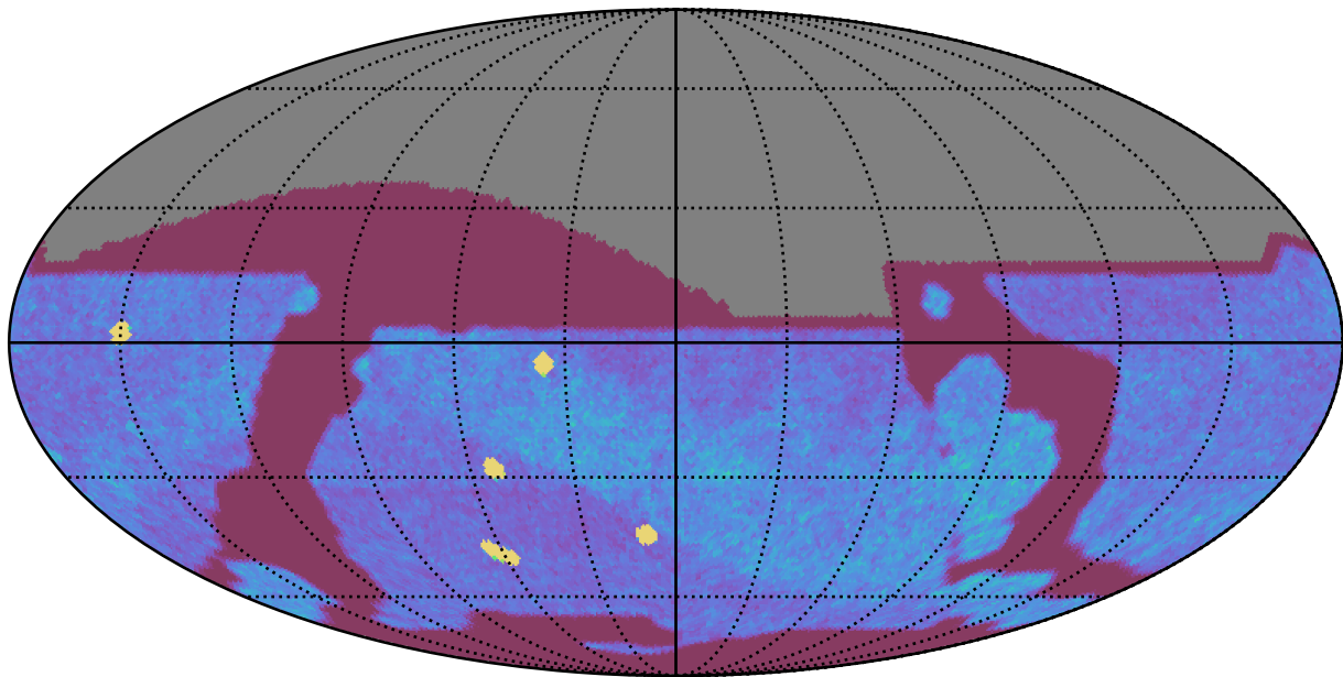
smc_lmc_v3.3_10yrs All sky z band: NVisits
