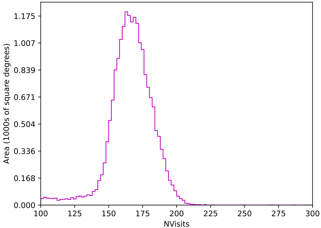
smc_lmc_v3.3_10yrs All sky z band: NVisits
