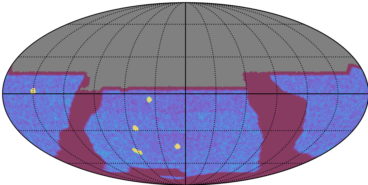
smc_lmc_v3.3_10yrs All sky y band: NVisits
