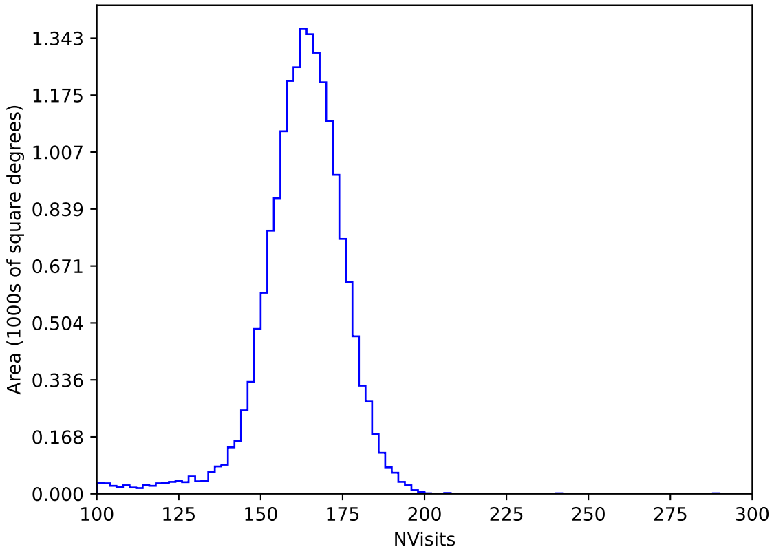
smc_lmc_v3.3_10yrs All sky y band: NVisits
