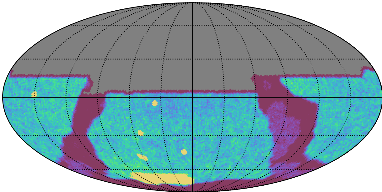
smc_lmc_v3.3_10yrs All sky u band: NVisits
