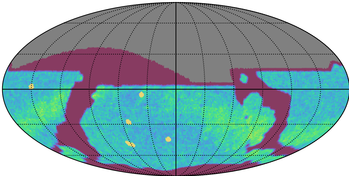
smc_lmc_v3.3_10yrs All sky r band: NVisits
