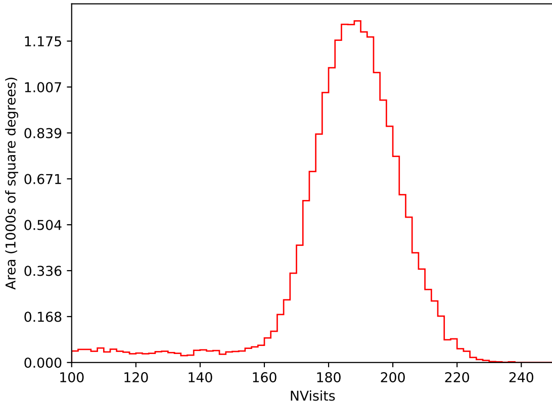
smc_lmc_v3.3_10yrs All sky i band: NVisits
