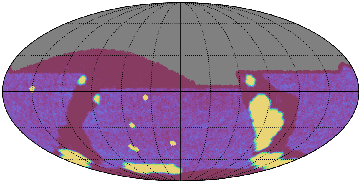
smc_lmc_v3.3_10yrs All sky g band: NVisits
