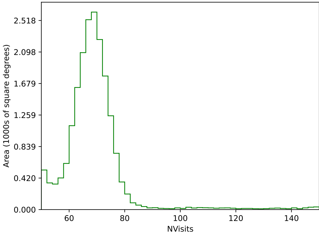
smc_lmc_v3.3_10yrs All sky g band: NVisits
