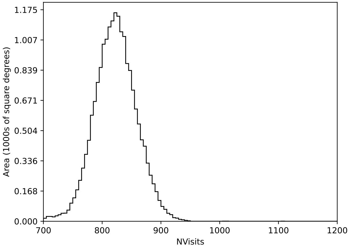
smc_lmc_v3.3_10yrs All sky all bands: NVisits
