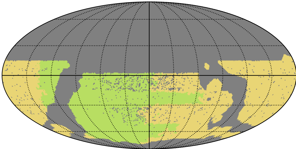
smc_lmc_v3.3_10yrs WFD all bands: NSeasons
