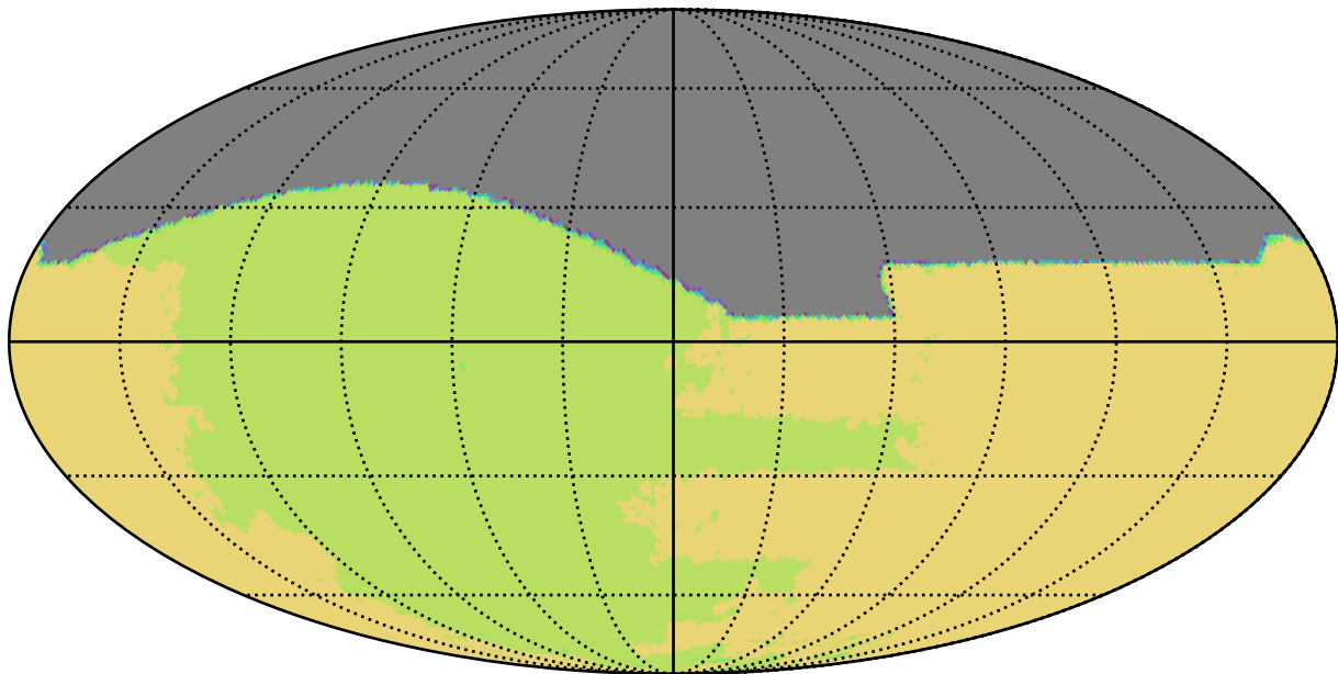
smc_lmc_v3.3_10yrs All sky all bands: NSeasons
