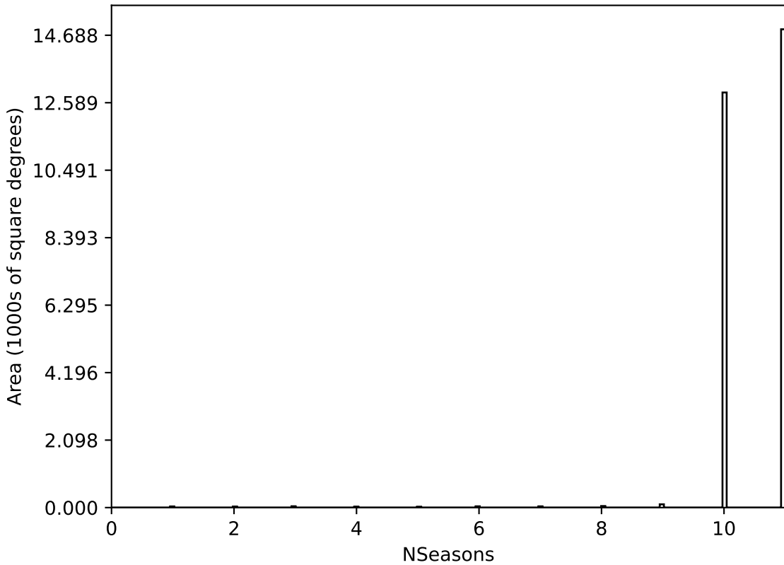
smc_lmc_v3.3_10yrs All sky all bands: NSeasons
