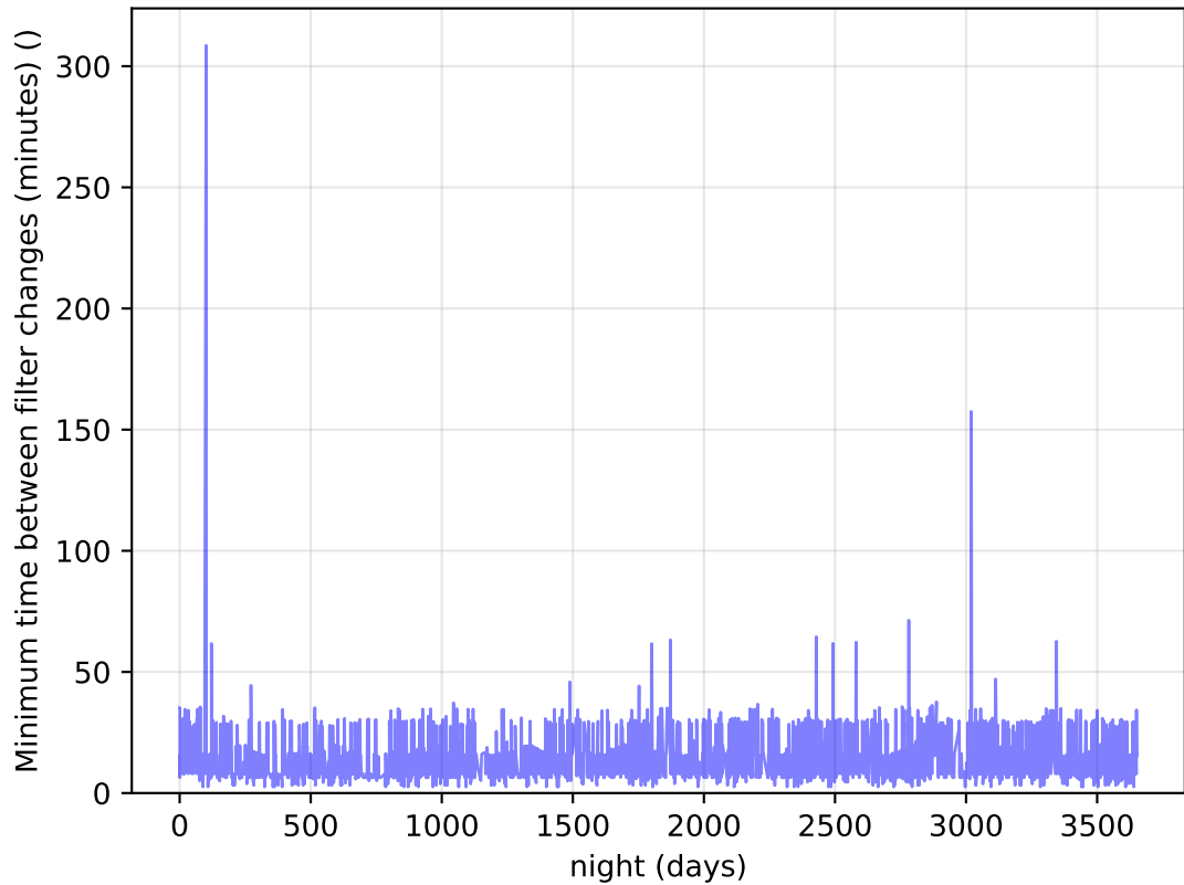
smc_lmc_v3.3_10yrs Per Night: Minimum time between filter changes (minutes)
