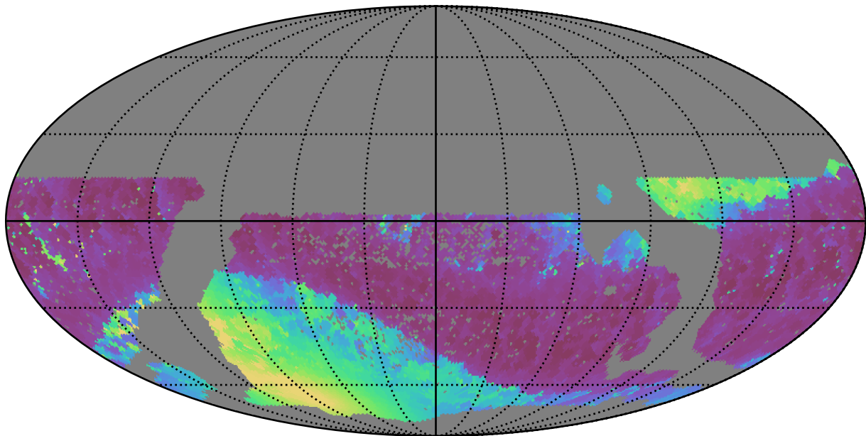
smc_lmc_v3.3_10yrs WFD z band: Min solarElong
