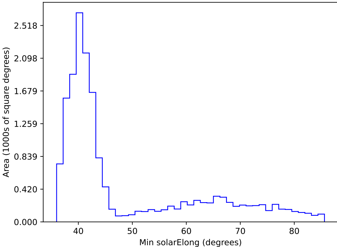
smc_lmc_v3.3_10yrs WFD z band: Min solarElong
