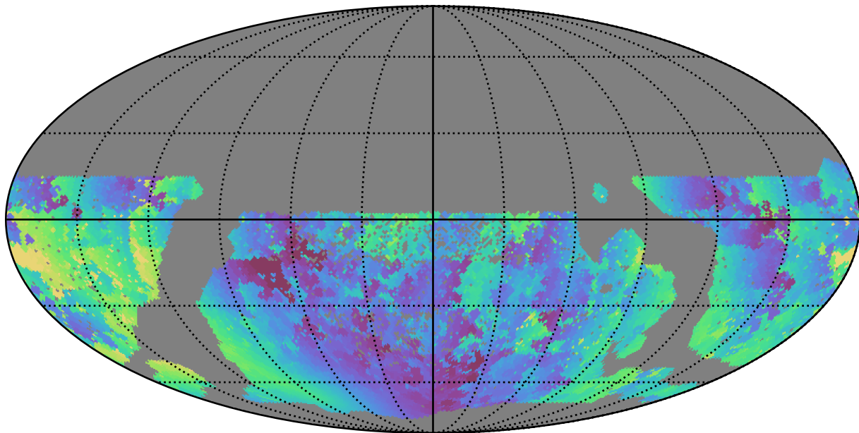
smc_lmc_v3.3_10yrs WFD u band: Min solarElong
