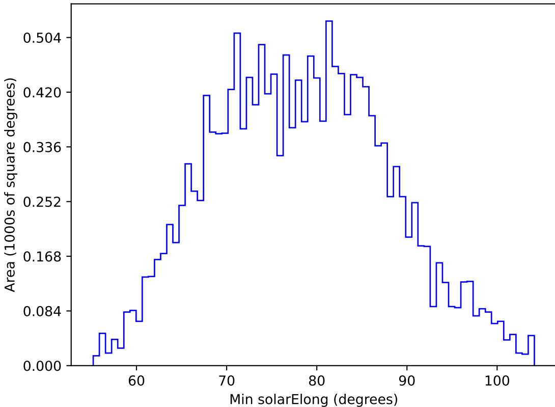
smc_lmc_v3.3_10yrs WFD u band: Min solarElong
