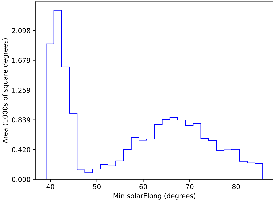
smc_lmc_v3.3_10yrs WFD r band: Min solarElong
