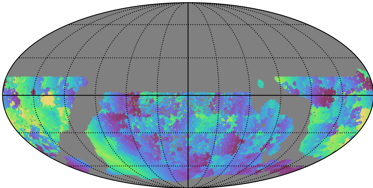
smc_lmc_v3.3_10yrs WFD g band: Min solarElong
