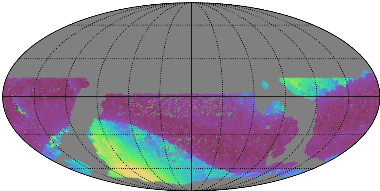
smc_lmc_v3.3_10yrs WFD all bands: Min solarElong
