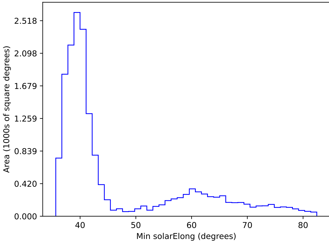
smc_lmc_v3.3_10yrs WFD all bands: Min solarElong
