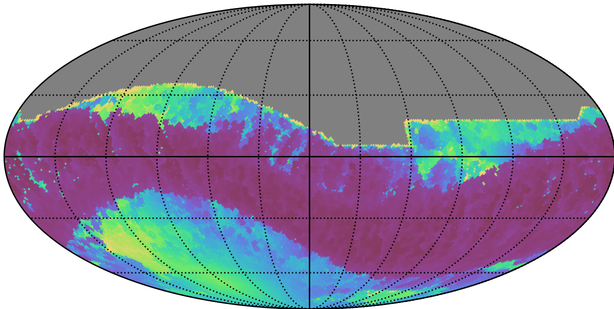
smc_lmc_v3.3_10yrs All sky z band: Min solarElong
