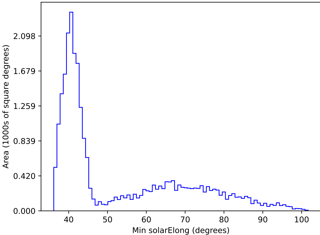
smc_lmc_v3.3_10yrs All sky z band: Min solarElong
