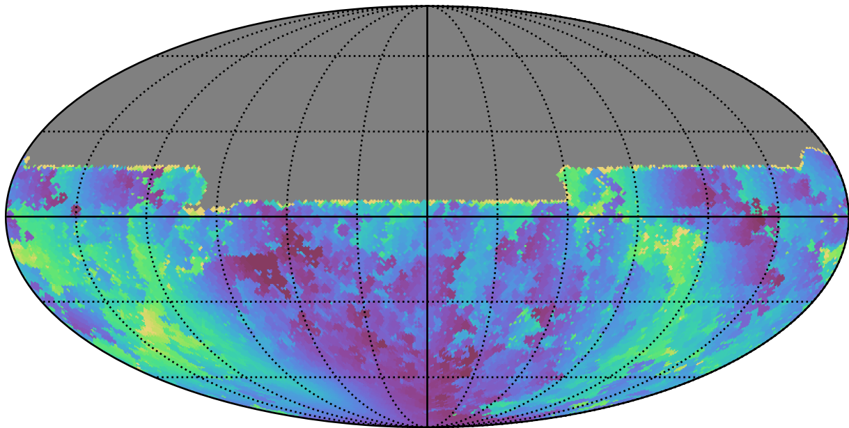
smc_lmc_v3.3_10yrs All sky u band: Min solarElong
