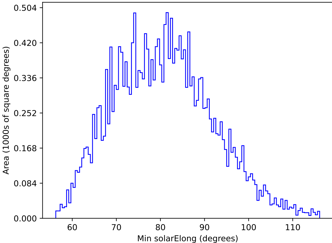
smc_lmc_v3.3_10yrs All sky u band: Min solarElong
