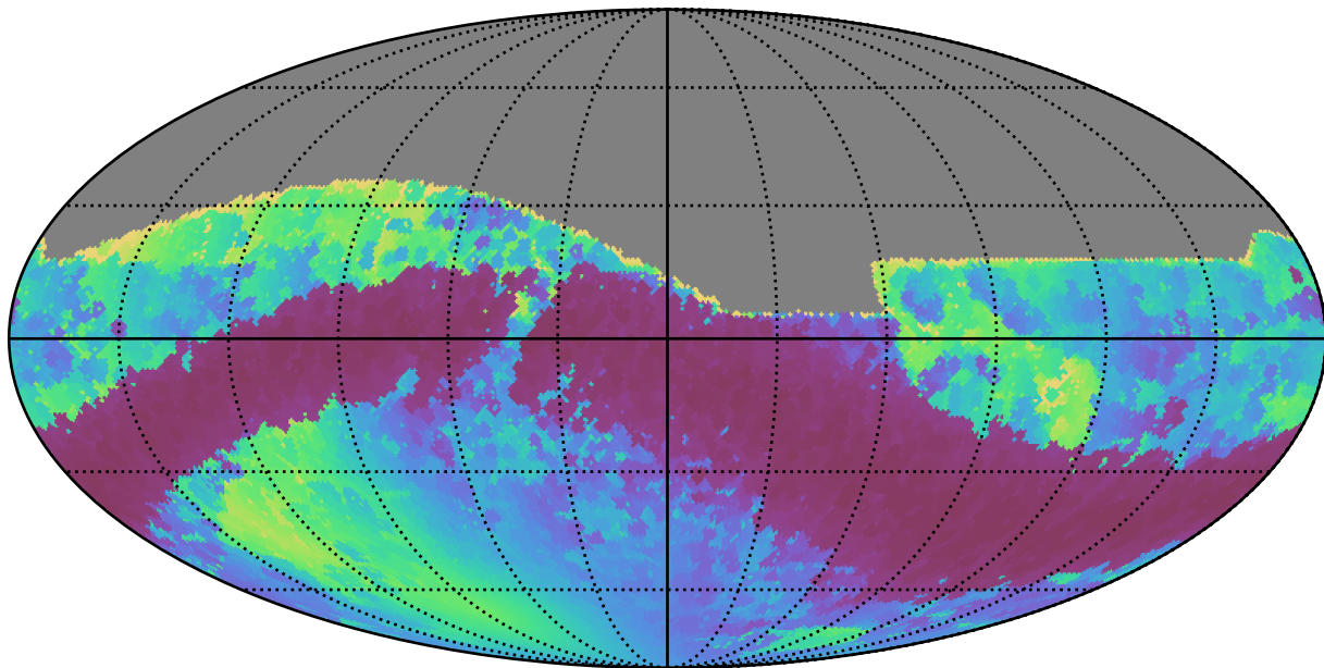
smc_lmc_v3.3_10yrs All sky r band: Min solarElong
