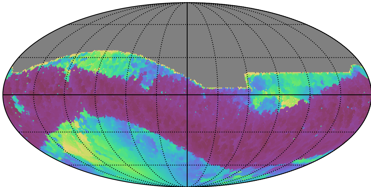
smc_lmc_v3.3_10yrs All sky i band: Min solarElong
