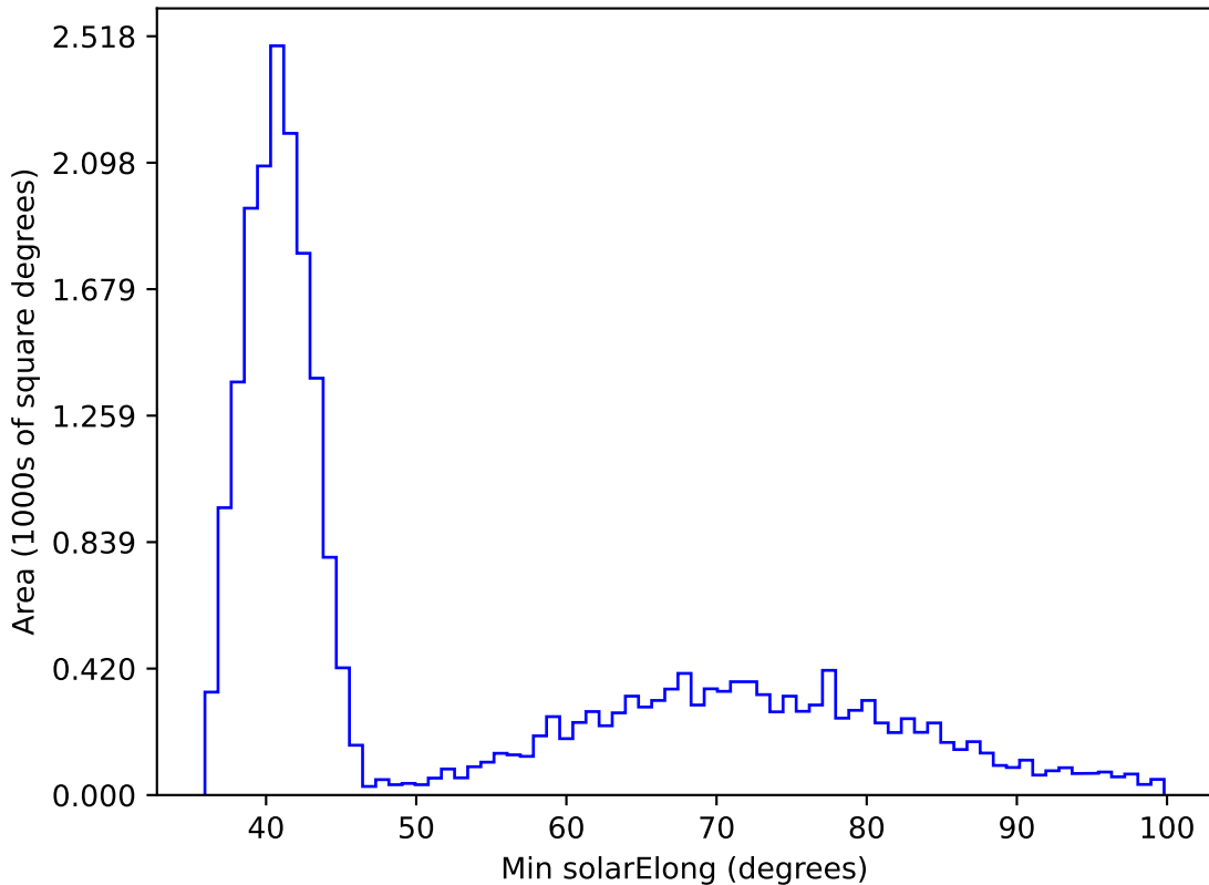
smc_lmc_v3.3_10yrs All sky i band: Min solarElong
