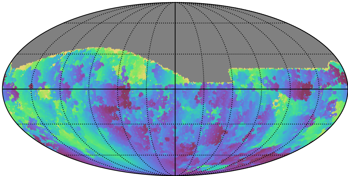
smc_lmc_v3.3_10yrs All sky g band: Min solarElong
