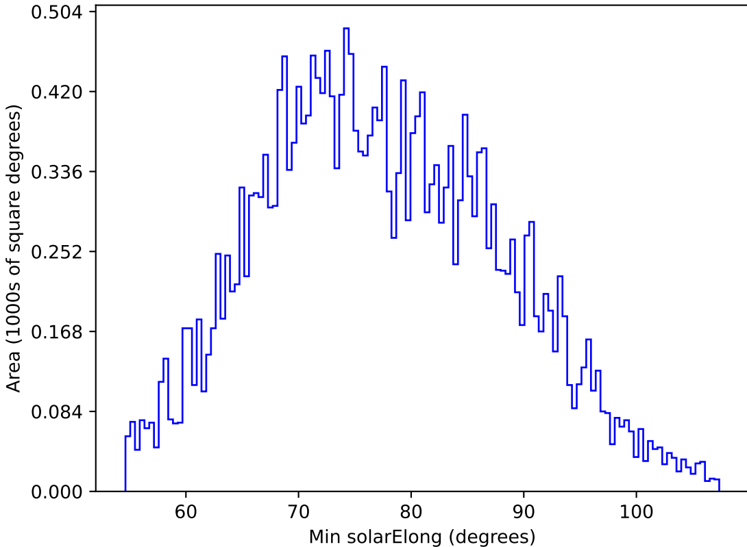
smc_lmc_v3.3_10yrs All sky g band: Min solarElong
