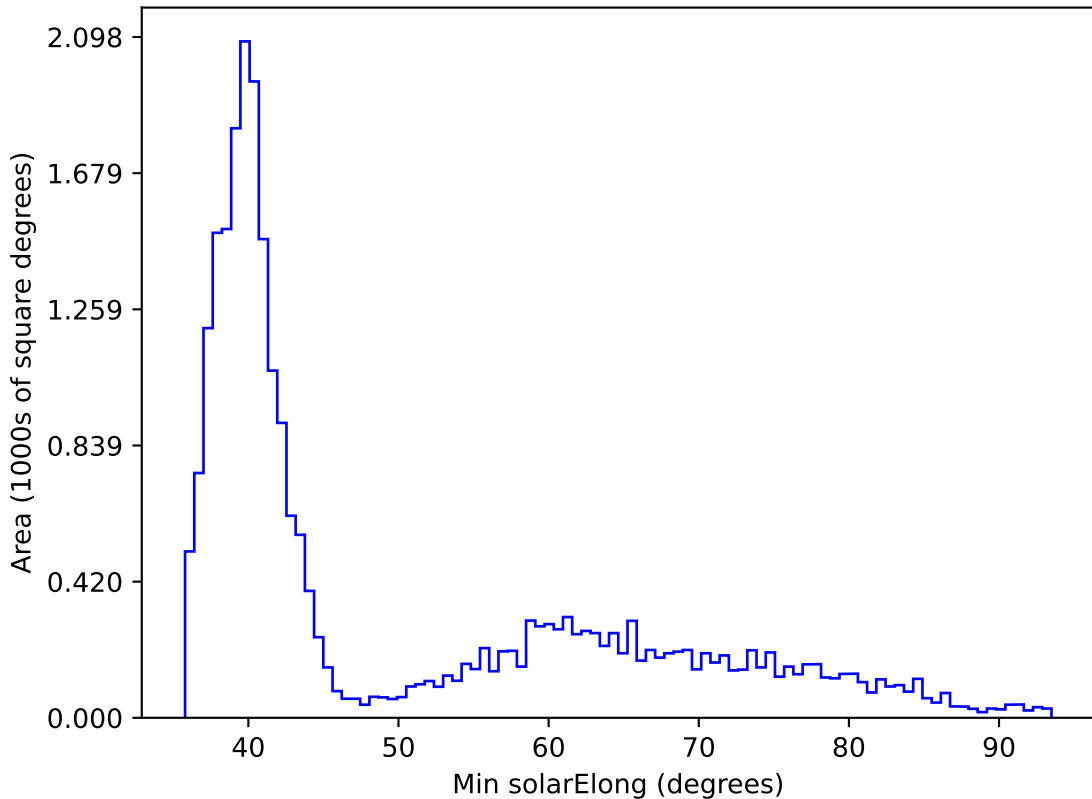
smc_lmc_v3.3_10yrs All sky all bands: Min solarElong
