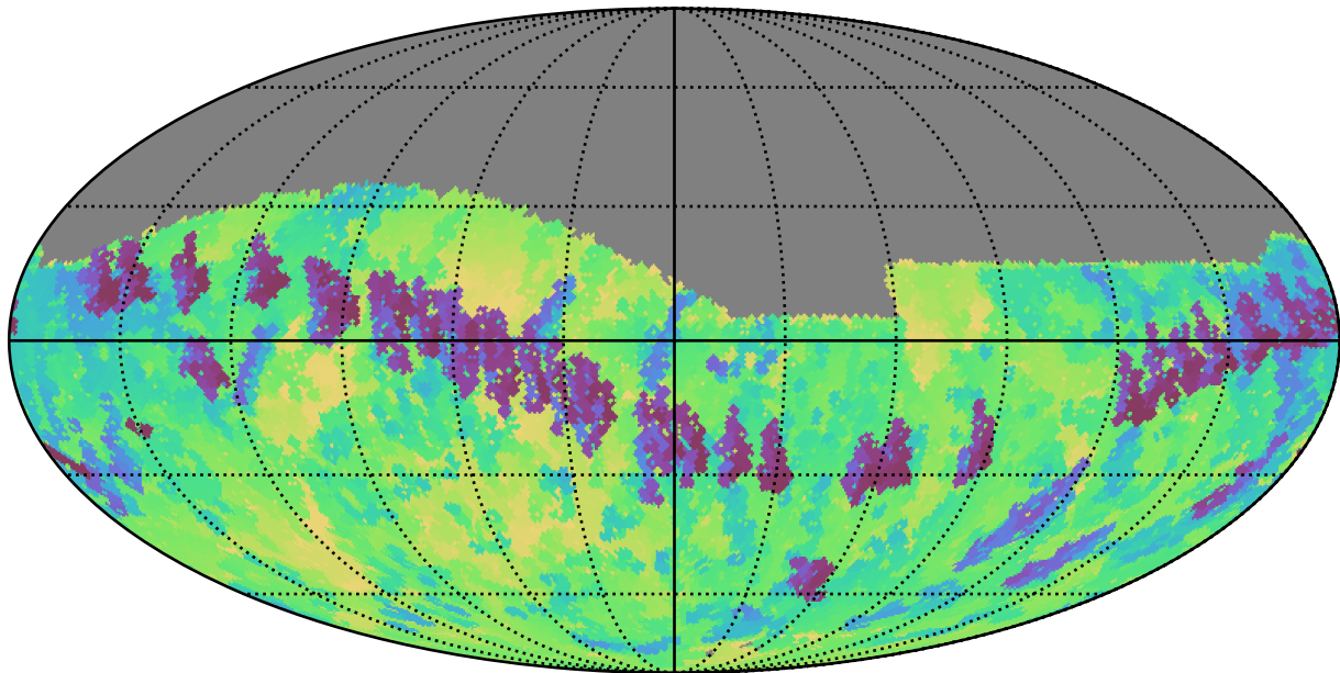
smc_lmc_v3.3_10yrs Yr 1 z band: Min skyBrightness
