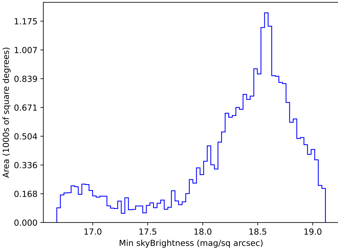
smc_lmc_v3.3_10yrs Yr 1 z band: Min skyBrightness
