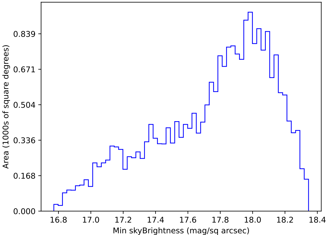
smc_lmc_v3.3_10yrs Yr 1 y band: Min skyBrightness
