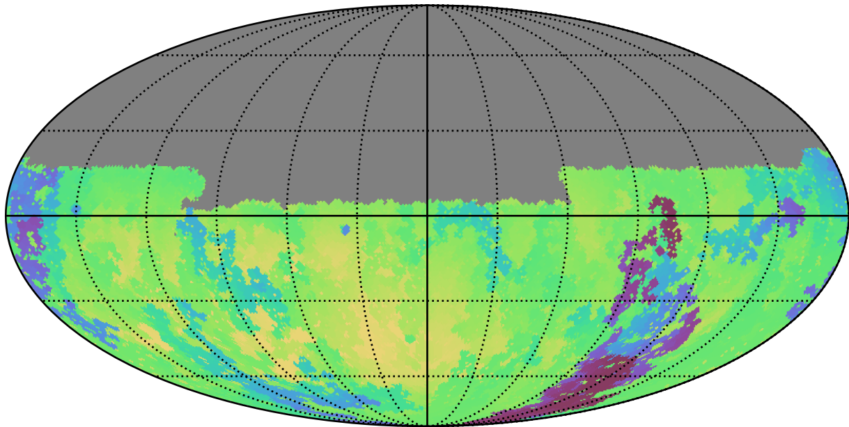
smc_lmc_v3.3_10yrs Yr 1 u band: Min skyBrightness
