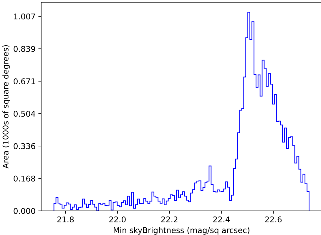
smc_lmc_v3.3_10yrs Yr 1 u band: Min skyBrightness
