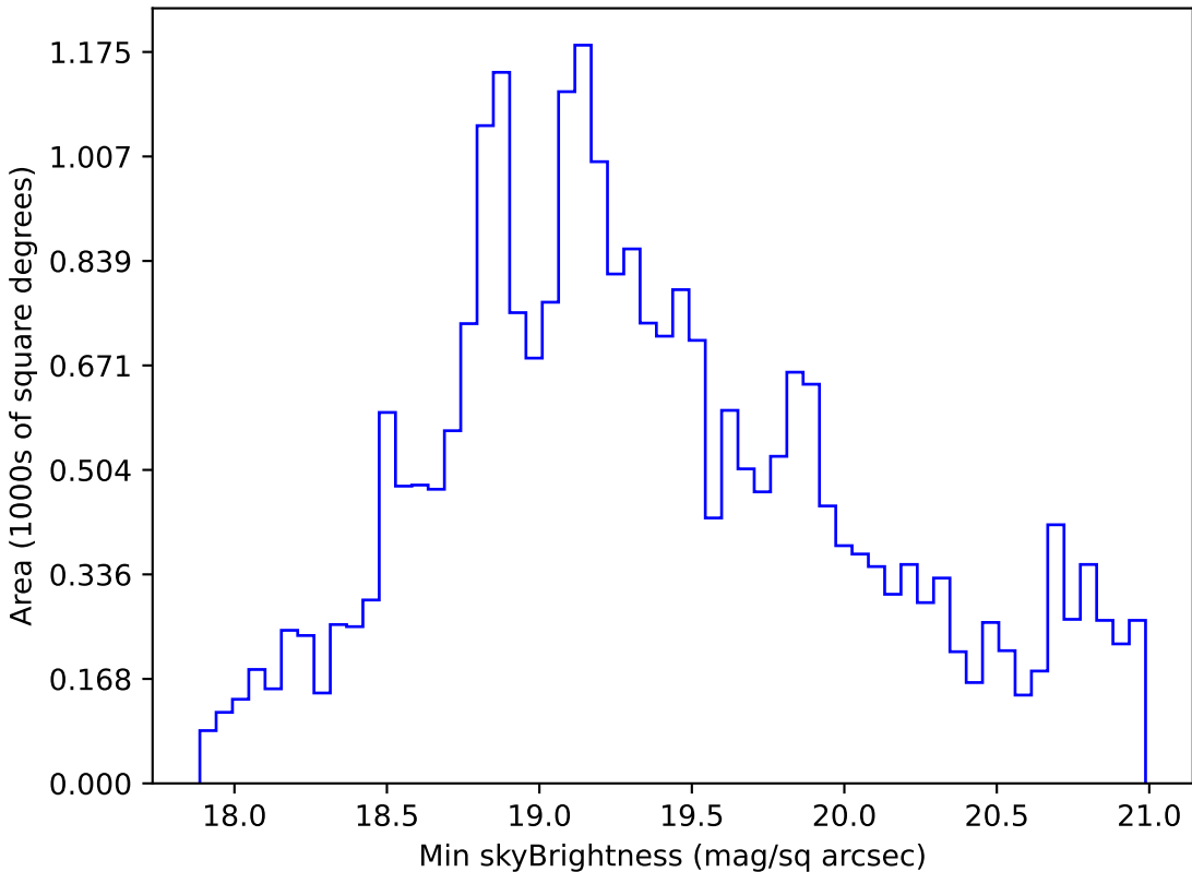
smc_lmc_v3.3_10yrs Yr 1 r band: Min skyBrightness
