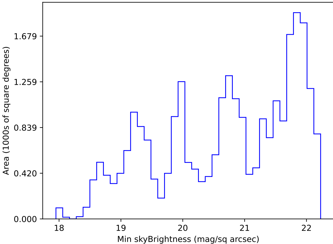
smc_lmc_v3.3_10yrs Yr 1 g band: Min skyBrightness
