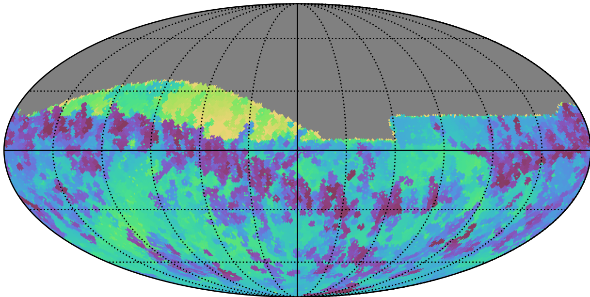
smc_lmc_v3.3_10yrs Yr 1 all bands: Min skyBrightness
