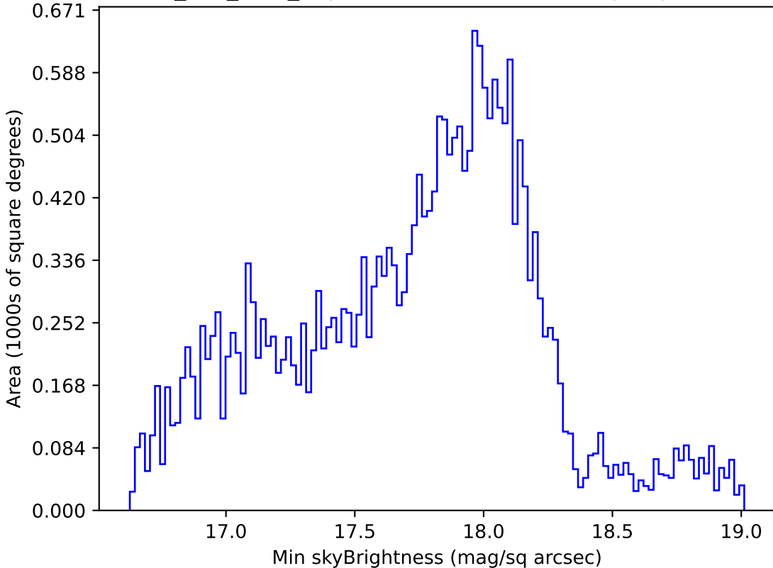
smc_lmc_v3.3_10yrs Yr 1 all bands: Min skyBrightness
