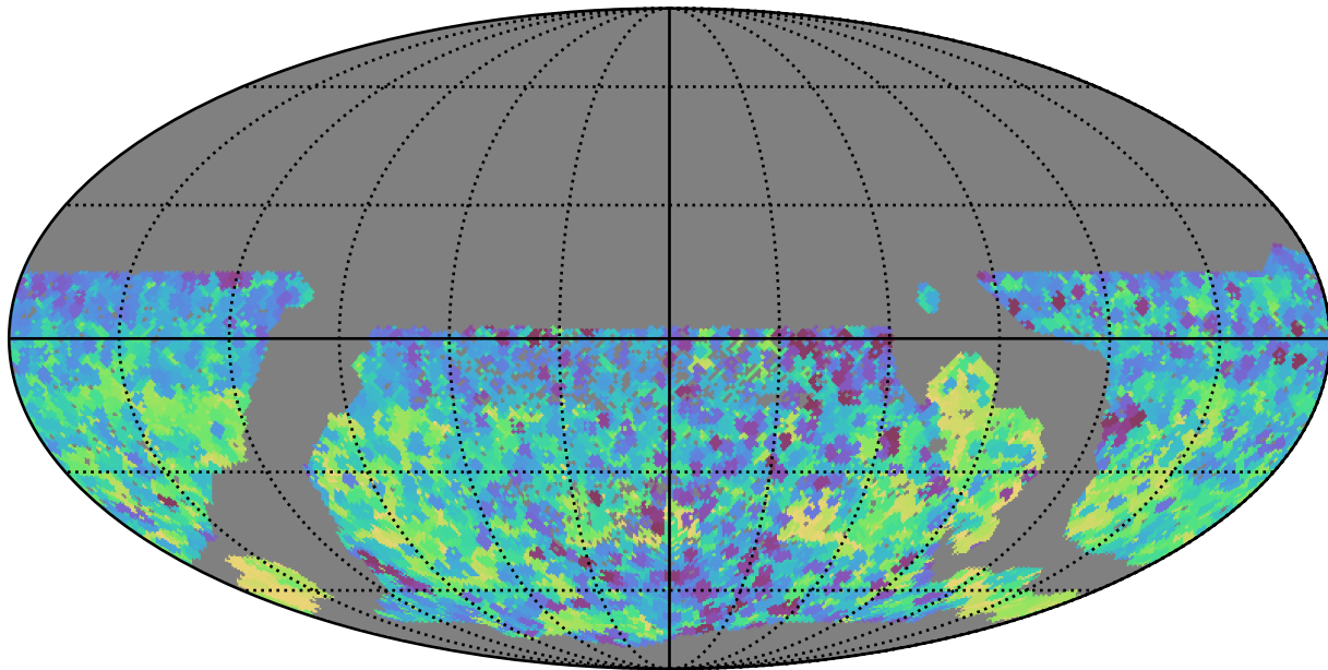
smc_lmc_v3.3_10yrs WFD y band: Min skyBrightness
